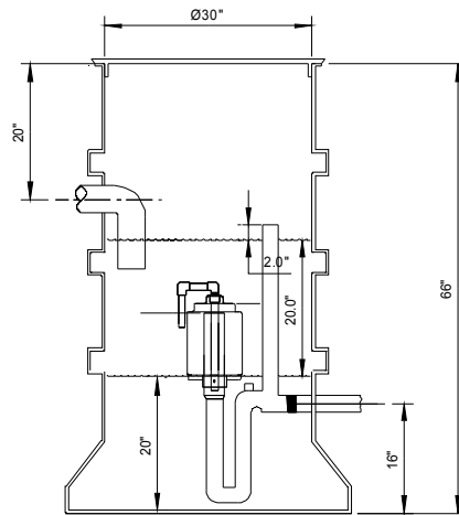
SIPHON BASIN
