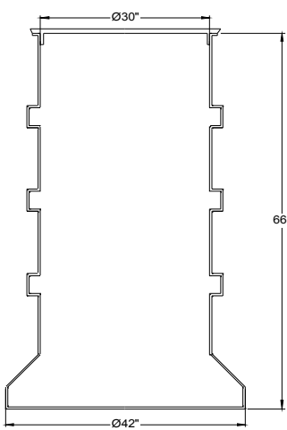
PUMP BASIN
